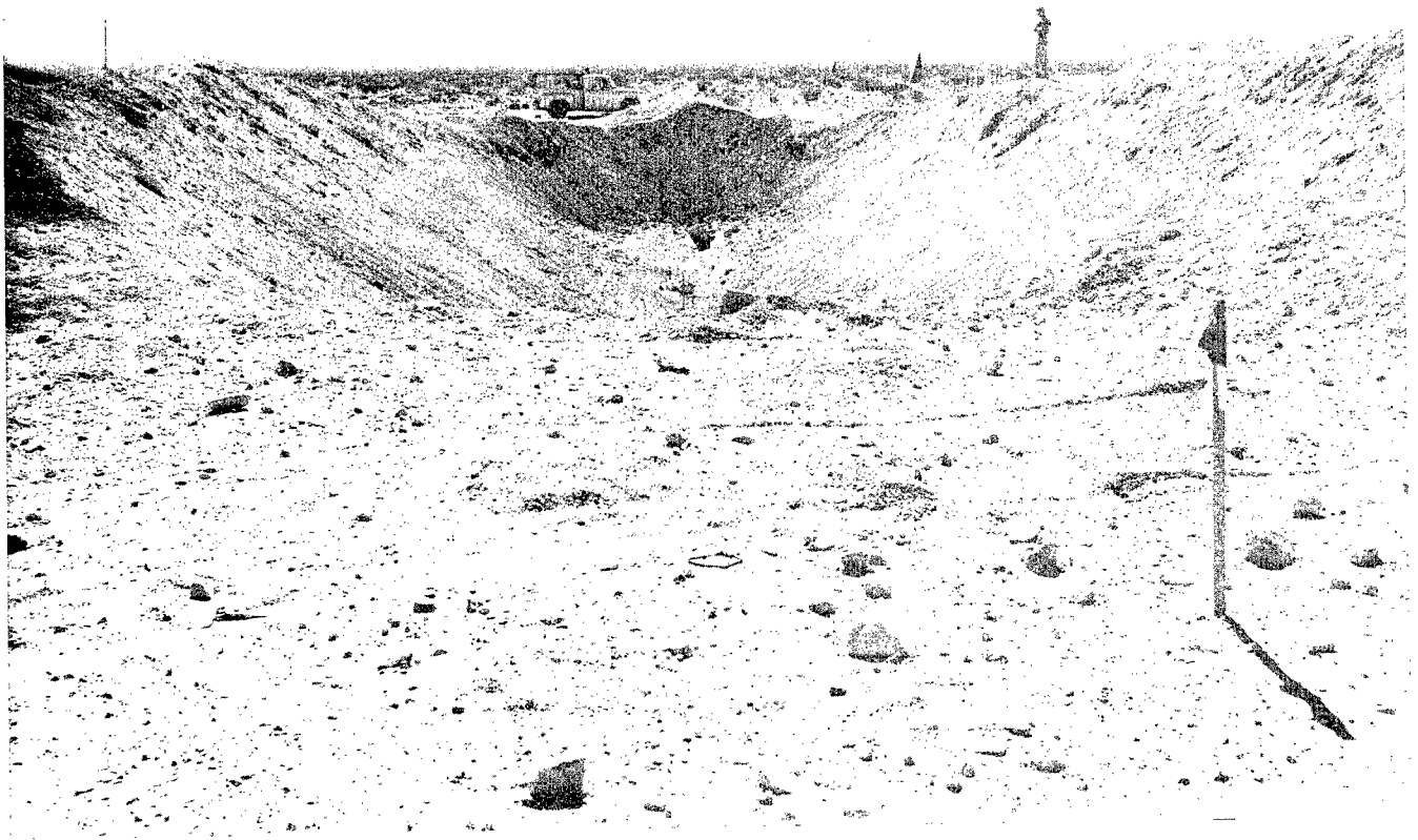
Fig. 17. End view of Pre-Buggy crater showing high side lip and absence of lip on the end.
